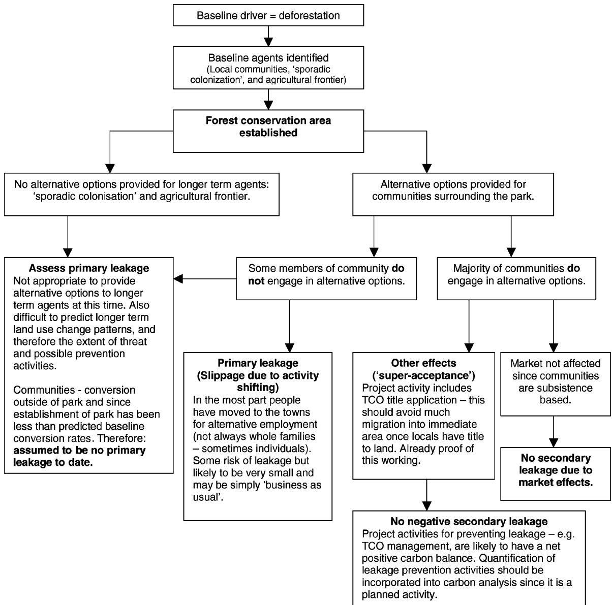
Fig. 2. Decision tree applied to the Noel Kempff Project. (‘Tierras Comunitarias de Origen’ (TCO)—grants land management rights to indigenous groups. A detailed natural resource management plan is required.)
